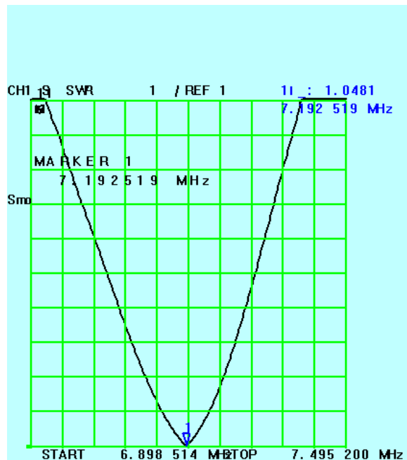
Fig. 2: Measured VSWR on The HP VNA
