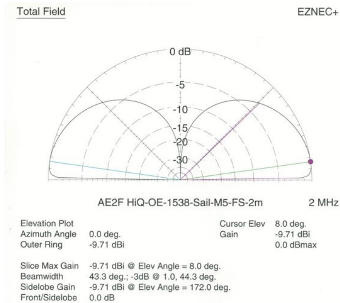
Hi-Q-6 OE-1538 mounted in the mast fully extended , Computed Radiation Pattern and Gain
