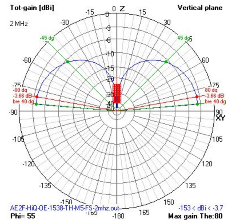
Plot of the Hi-Q-5-2-30 MHz submarine antenna.
